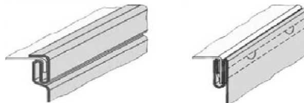
Pittsburgh Lock Seam
